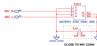
Mic Conn
